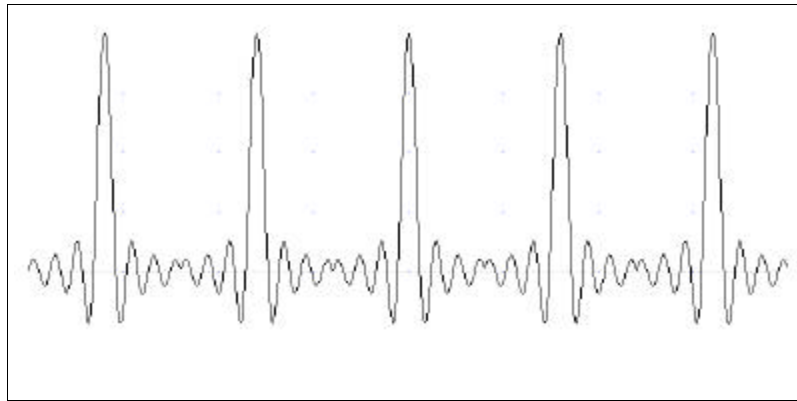
Figure 1-1 Segment 1 - Sin(x)/x Waveform
